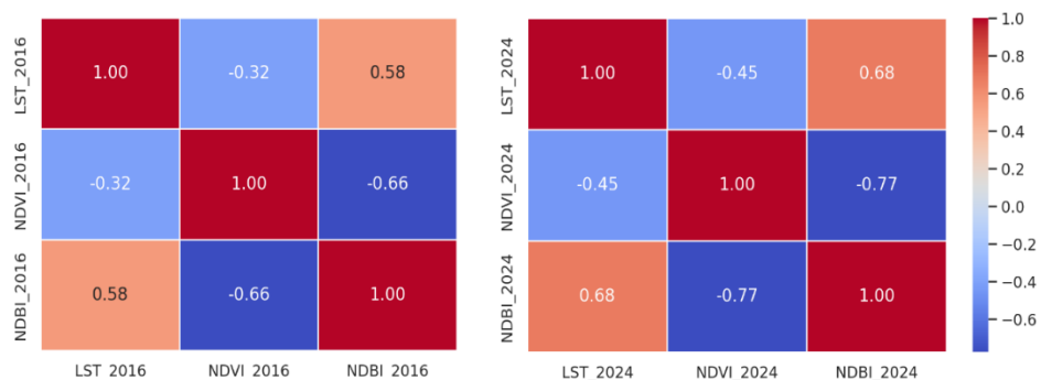
Figure 4: Correlation Matrix among LST, NDVI, and NDBI in 2016 and 2024
