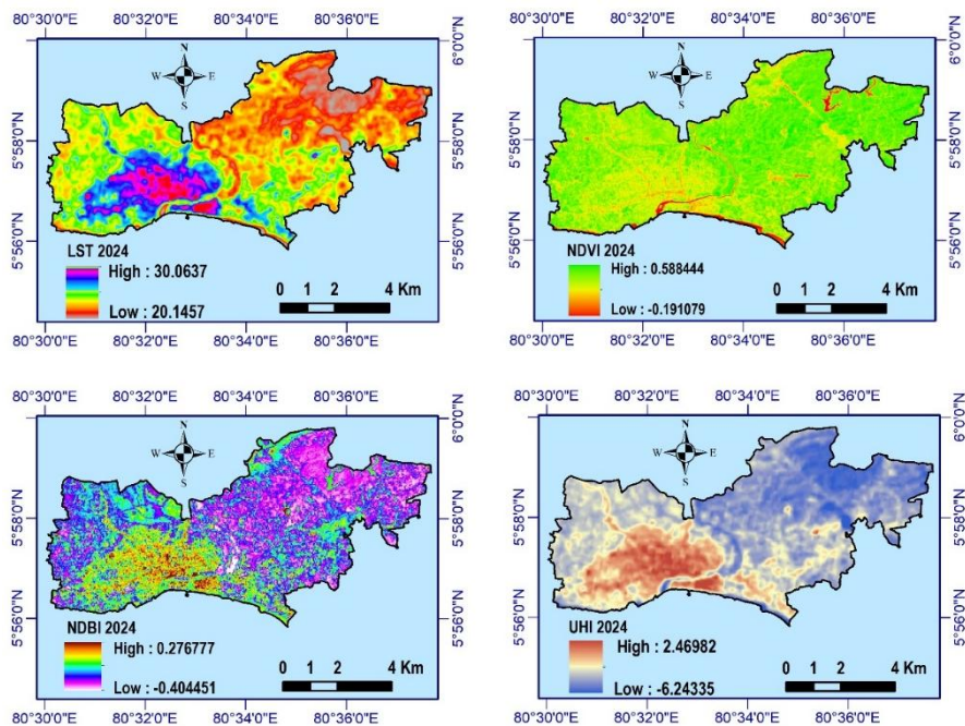
Figure 3: LST, NDVI, NDBI and UHI in 2024
