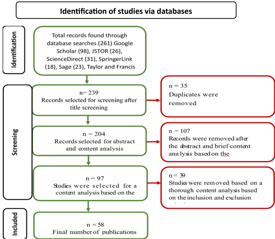
Figure 2: Methodological coverage
